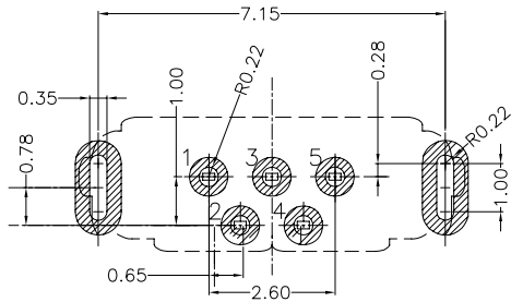
PASTE-IN-HOLE RECOMMENDED P.C.B LAYOUT
