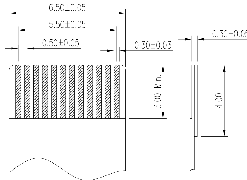
RECOMMEND P.C.B. PATTERN DIMENSION(TOP VIEW)
