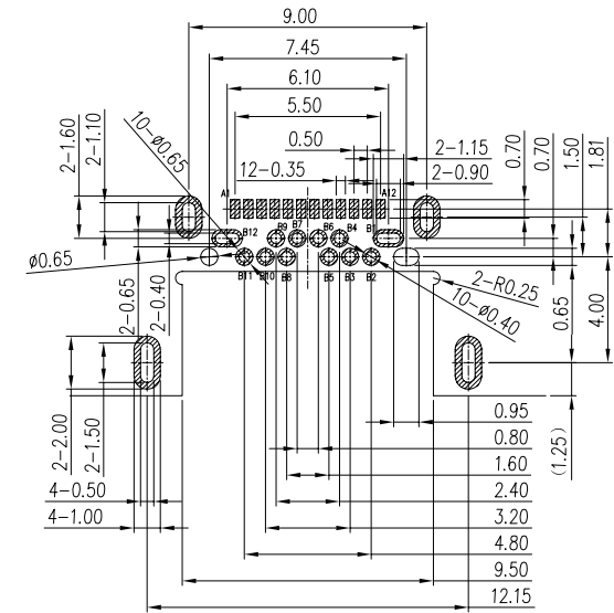
RECOMMEND P.C.B LAYOUT (COMPONENT SIDE) TOLERANCE: ±0.05
